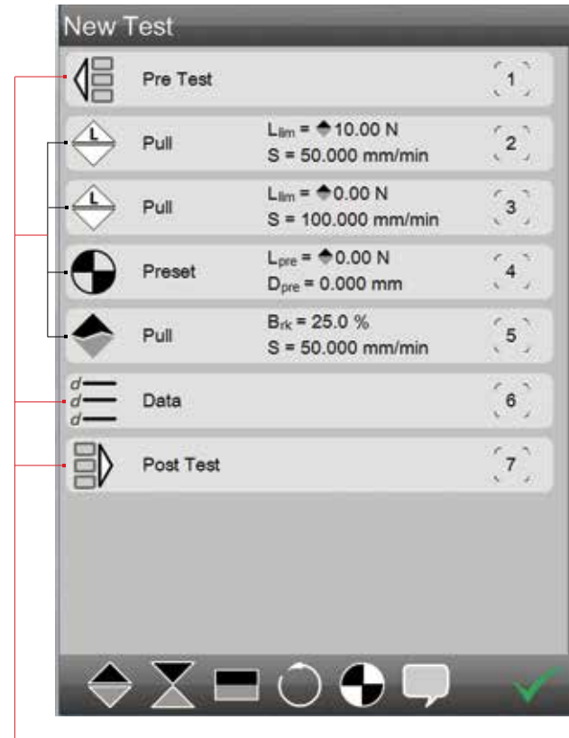
Test setups are comprised of four stages: Pre Test, Test, Data and Post Test.
